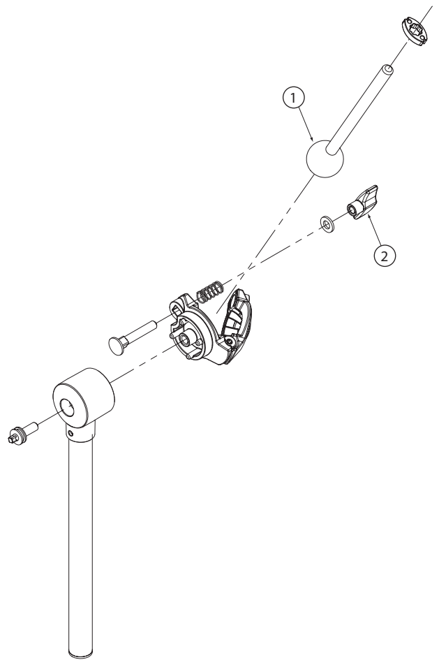
Exploded View (Fig.4)
