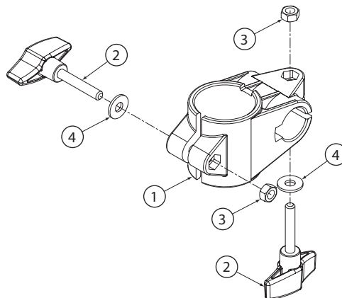
Exploded View (Fig.8)
