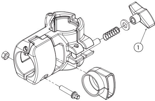
Exploded View (Fig.1)
