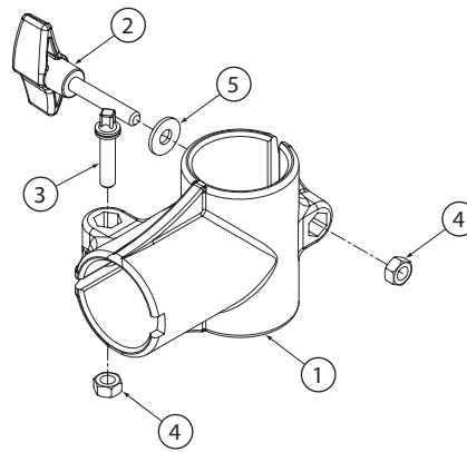
Exploded View (Fig.7)
