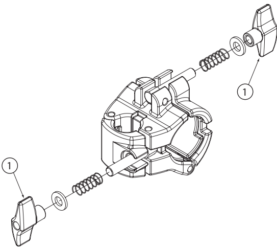
Exploded View (Fig.2)
